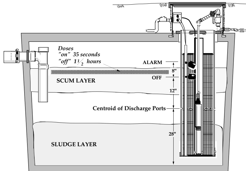
Figure 6: Float Levels in a 1500 Gallon Tank Serving Four Occupants.
