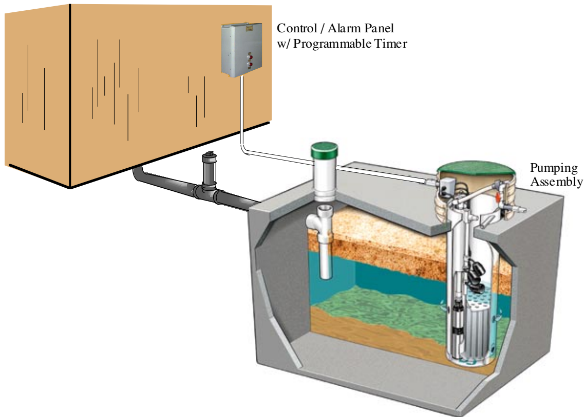
Figure 1: Septic Tank and Pumping Assembly
