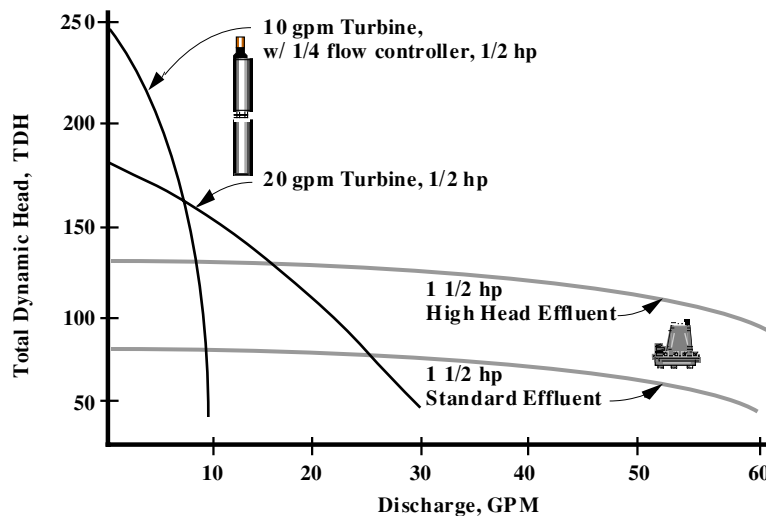
Figure 9: Effluent Pump Options
