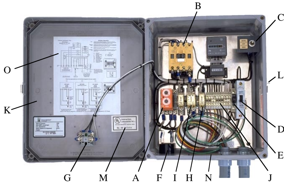
Figure 3: Simplex Control Panel with Programmable Timer
