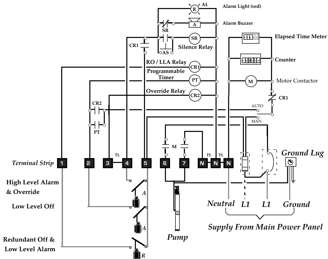
Figure 4: Control Panel Wiring Schematic
