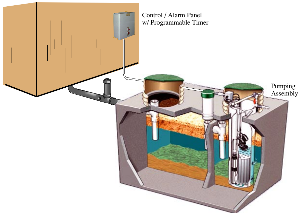
Figure 2: Dual Compartment Septic Tank with Pumping Assembly
