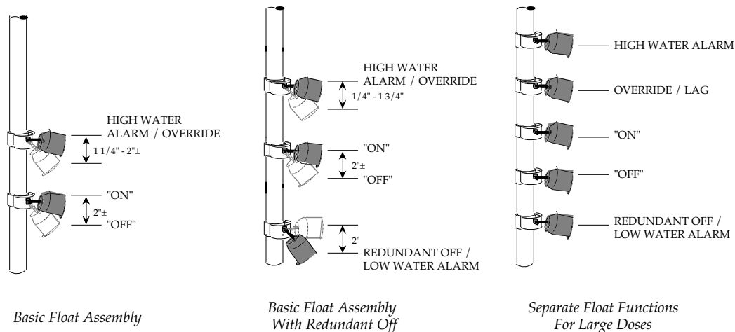
Figure 5: Level Control Float Assemblies
