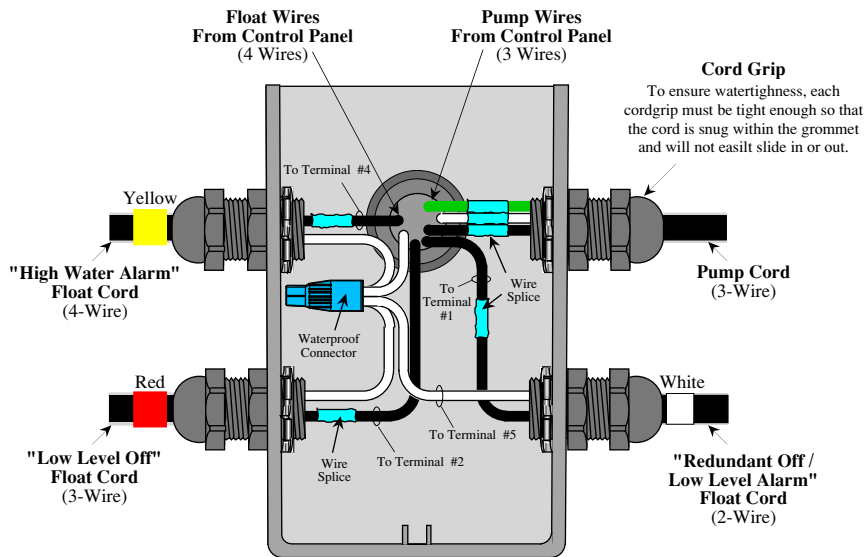
Figure 7: Electrical Splice Box Assembly
