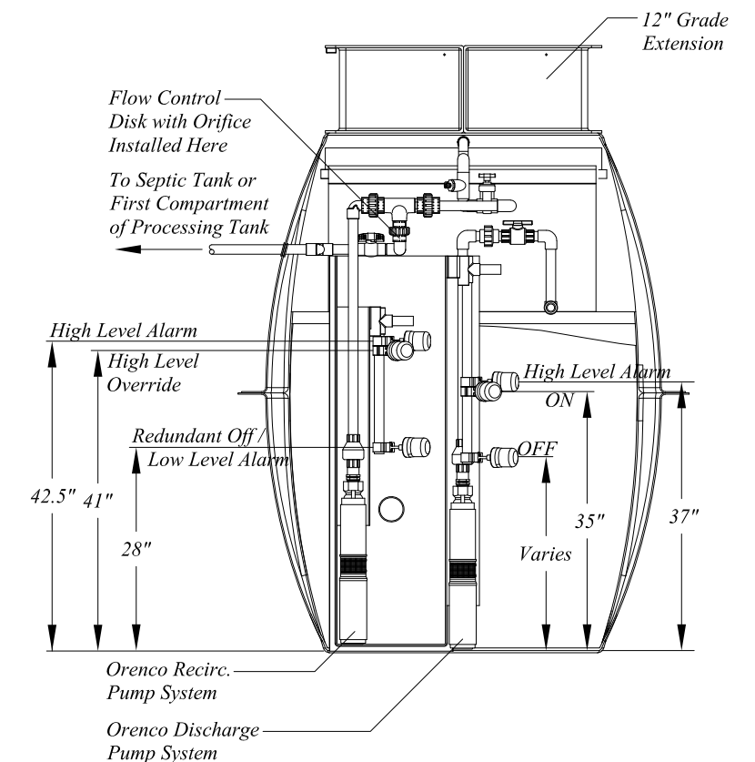
Discharge Chamber - End View
