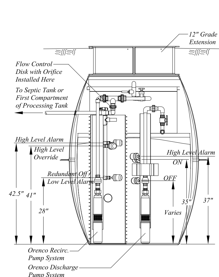
Discharge Chamber - End View
