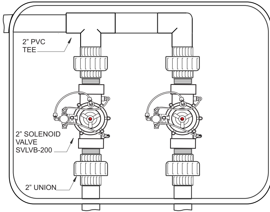
GEOFLOW 2" ZONE VALVE BOX - SVLVB200 X 2
