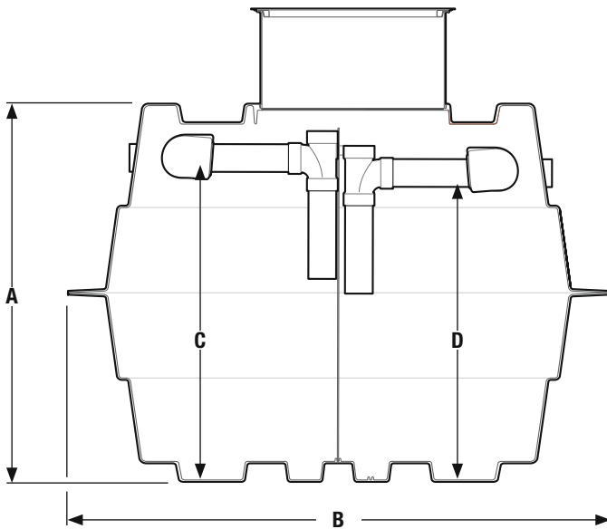
Side sectional view, M1000G (access riser and lid sold separately)
