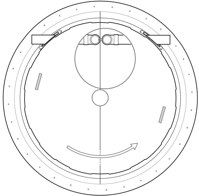
Top sectional view, M1000G
