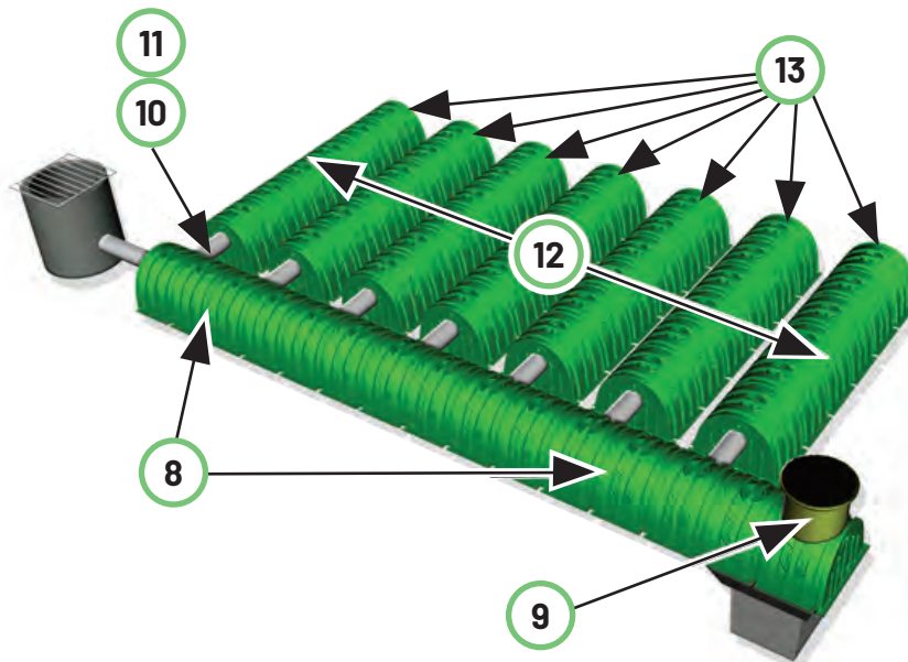
FIGURE 3 - Distribution Pipes
