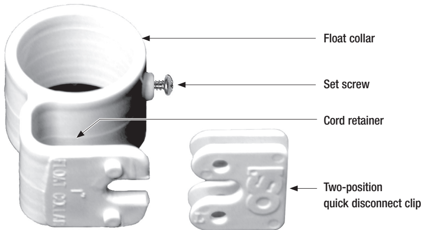
Orenco 1" Float Collar Kit
