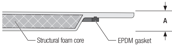
Orenco® FBL-Series Fiberglass Lid (close-up, side-cutaway view)
