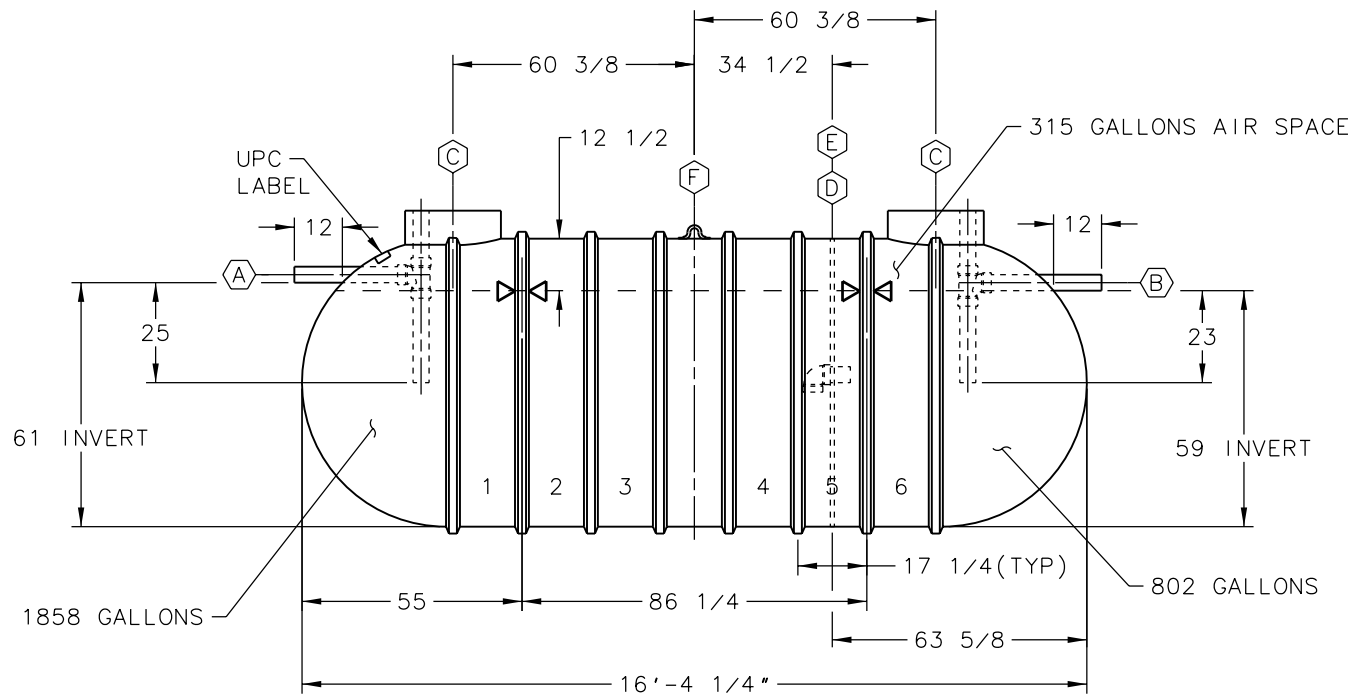
CROSS-OVER & BAFFLE DETAIL
