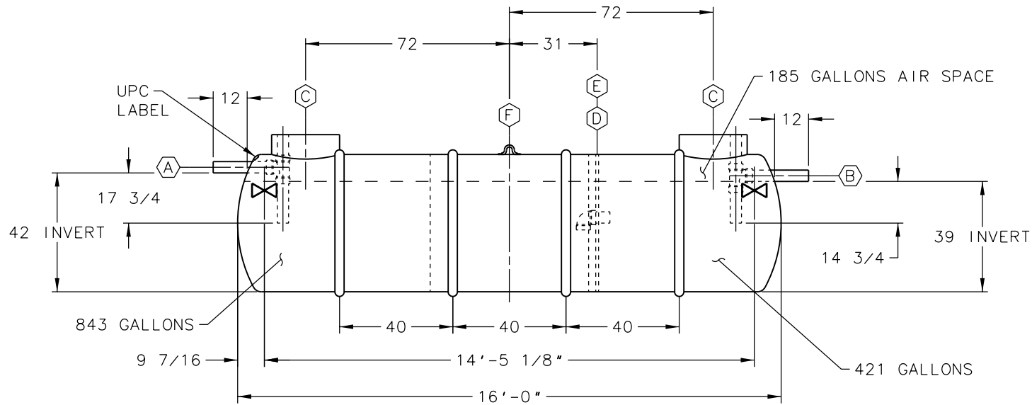
CROSS-OVER & BAFFLE DETAIL
