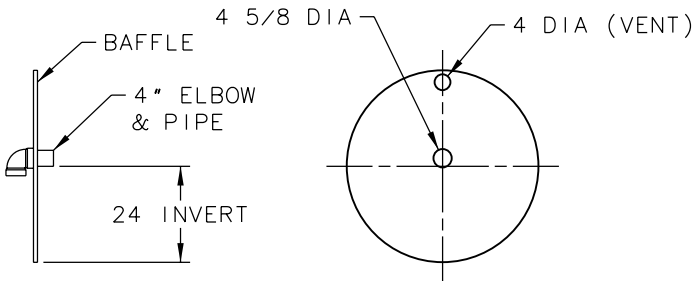
CROSS-OVER & BAFFLE DETAIL
