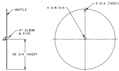
CROSS-OVER & BAFFLE DETAIL
