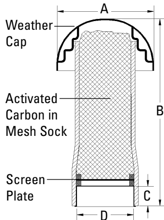
Cutaway View (side)
